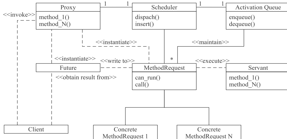
Rysunek 2: Źródło: D. C. Schmidt Pattern-Oriented Software Architectures for Concurrent and Networked Mobile Devices and Clouds D. C. Schmidt, M. Stal, H. Rohnert, F. Buschmann, Pattern-Oriented Software Architecture: Patterns for Concurrent and Networked Objects, Wiley & Sons, 2000
