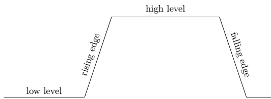
Figure 2: Binary Signal
