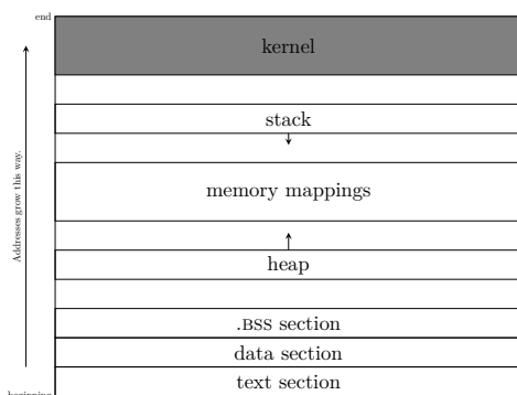
Figure 1: Conceptual Model of User Process Address Space in Linux
