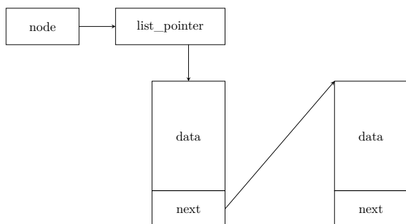
Before the line no. 6 of the delete_node() is performed
