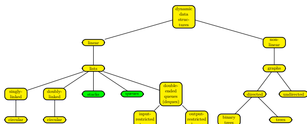
Classification of data structures
