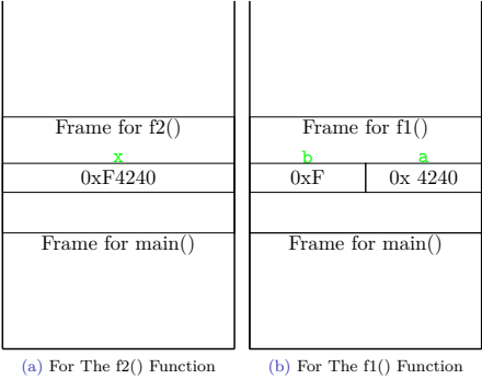
Figure: How The Frames Are Created on The Stack
